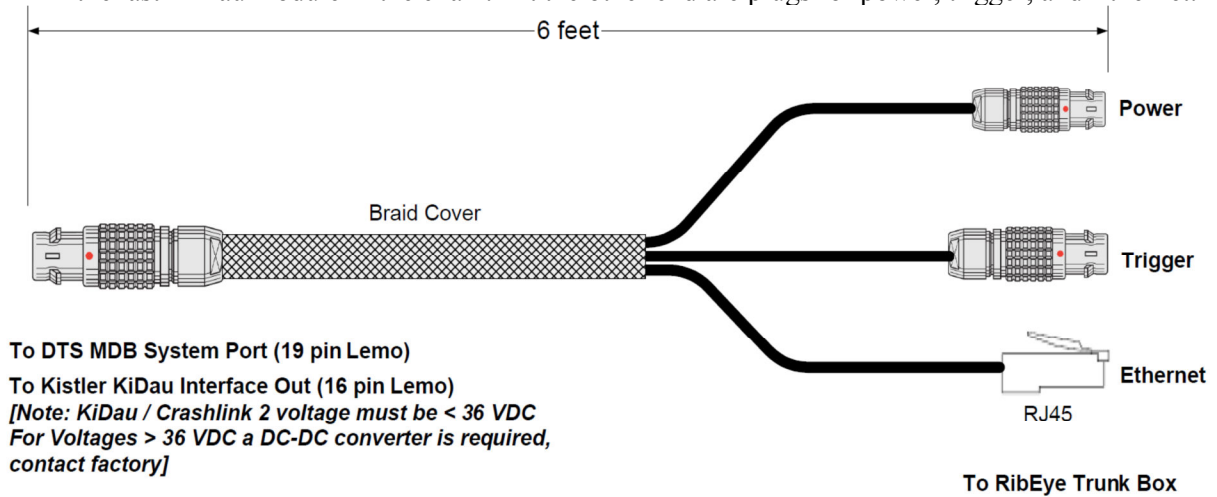
Figure 10. Cable assemblies for connecting Hybrid III RibEye to data acquisition systems
